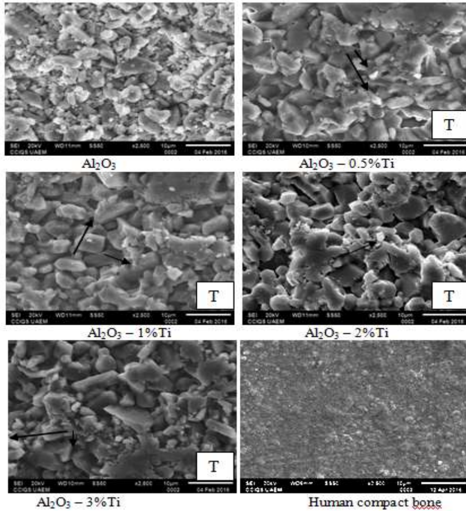
Fig. 4: Microstructure of composites \text{Al}_2\text{O}_3 -X wt. % Ti, (X = 0.5, 1, 2 and 3), sintered at 1400^\circ\text{C} during 2h, and microstructure of human compact bone
