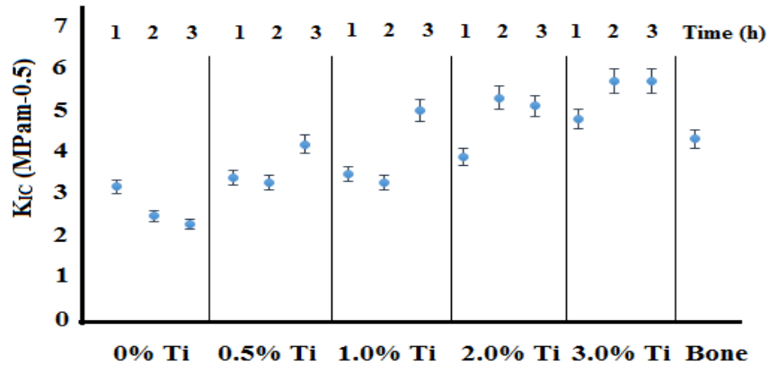
Fig. 2: Fracture toughness of composites Al 2 O 3 -X wt. % Ti, (X = 0.5, 1, 2 and 3), and fracture toughness of human compact bone
