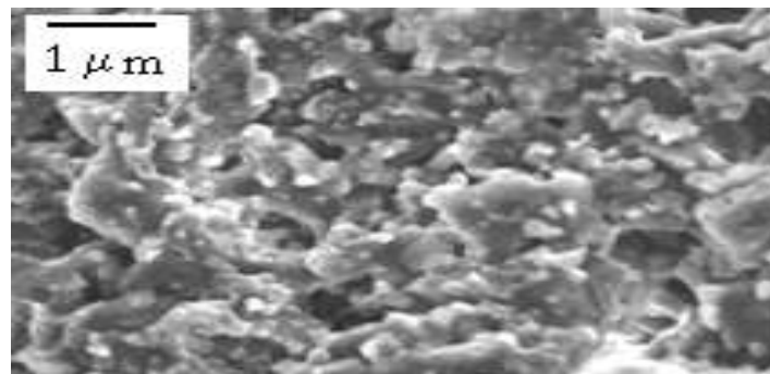
Fig. 7: Fracture surface in an Al 2 O 3 /Ti reinforced composite
