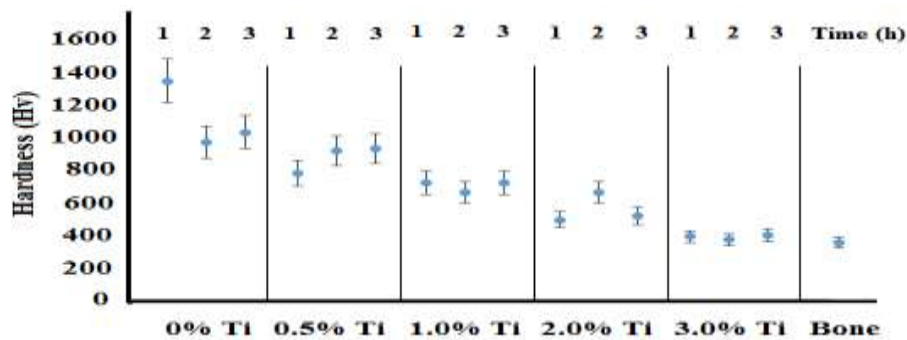
Fig. 3: Hardness of composites Al 2 O 3 -X wt. % Ti, (X = 0.5, 1, 2 and 3), and hardness of human compact bone
