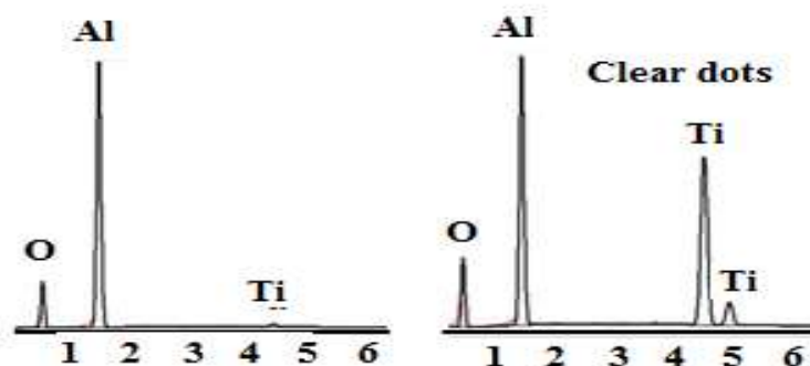
Fig. 5: EDX spectra corresponding to \text{Al}_2\text{O}_3 /0.0 wt % Ti and \text{Al}_2\text{O}_3 /3 wt % Ti sintered at 1400^\circ\text{C} for 2 hours
