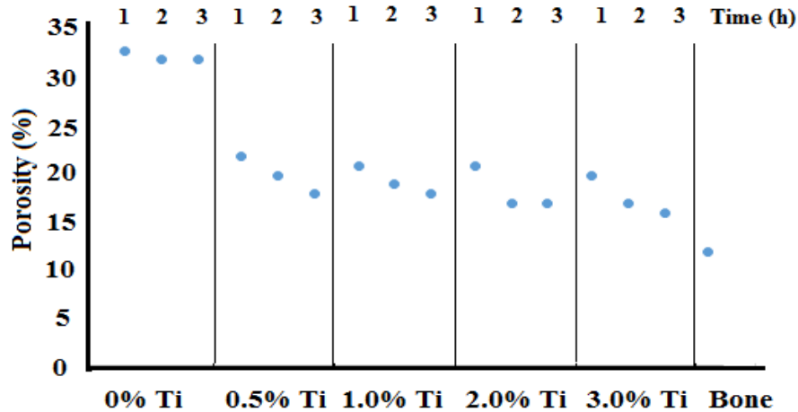
Fig. 1: Porosity of composites \text{Al}_2\text{O}_3\text{-X wt. \% Ti} , (X = 0.5, 1, 2 and 3), and porosity of human compact bone
